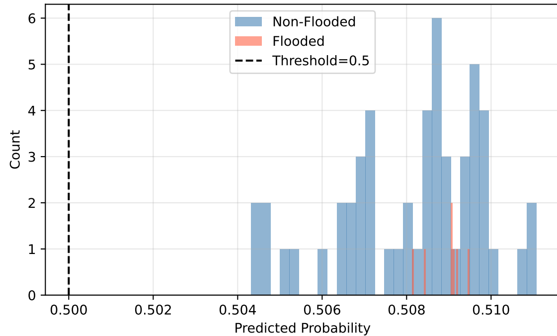
CustomCNN — Confidence Distribution
