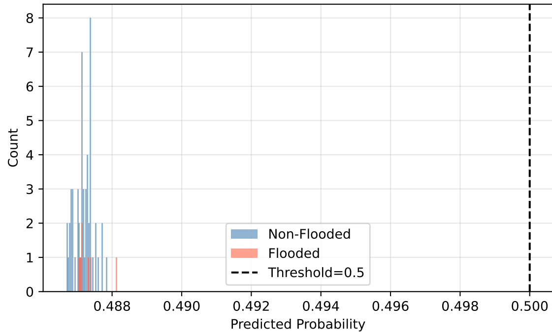
EfficientNetB0 — Confidence Distribution
